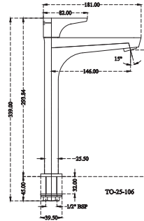
TO 25 106 | Pillar Cock Extension Body Long Nose with Base M.R.P. ₹ : 3675
