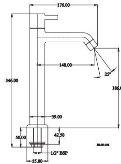
FR 09 106 | Pillar Cock Extension Body Long Nose with Base M.R.P. ₹ : 3775
