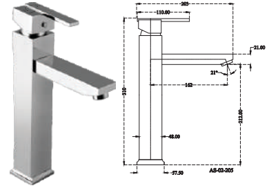
AS 02 205 | S/L Basin Mixer Extn. Body Without Pop Up 40mm Cartridge With 450mm Long Braided Hoses with Base M.R.P. ₹ : 9600
