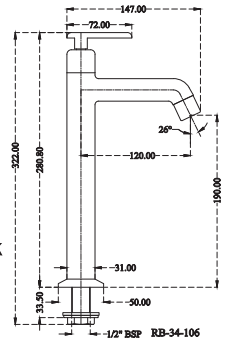
RB 34 106 | Pillar Cock Extension Body Long Nose with Base M.R.P. ₹ : 2795
