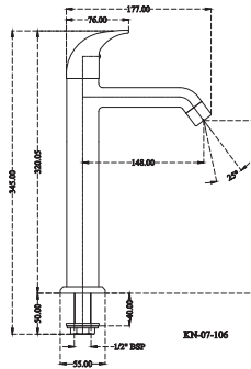
KN 07 106 | Pillar Cock Extension Body Long Nose with Base M.R.P. ₹ : 3845
